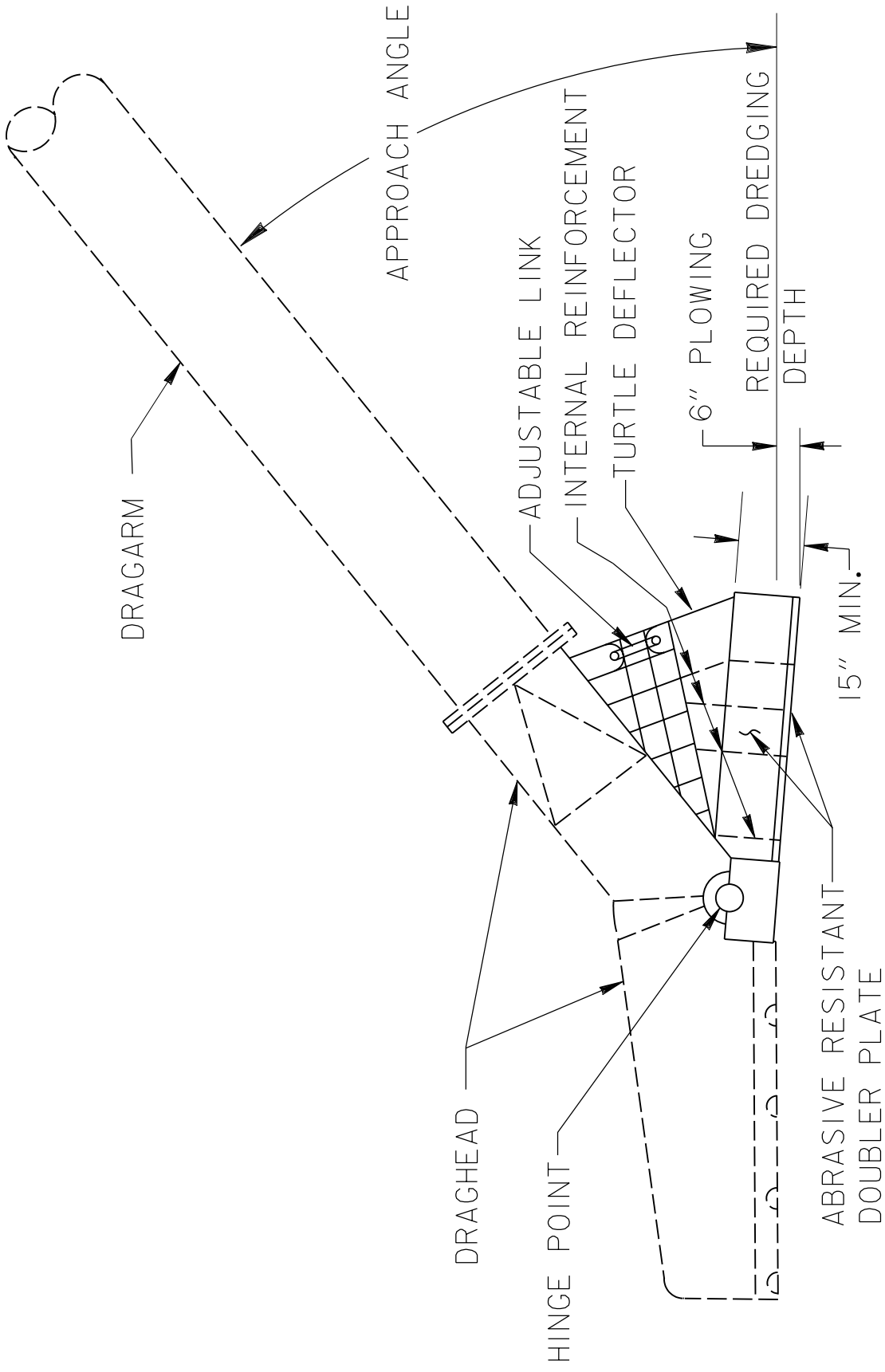
ELEVATION RIGID ADJUSTABLE TURTLE DEFLECTOR N.T.S.
