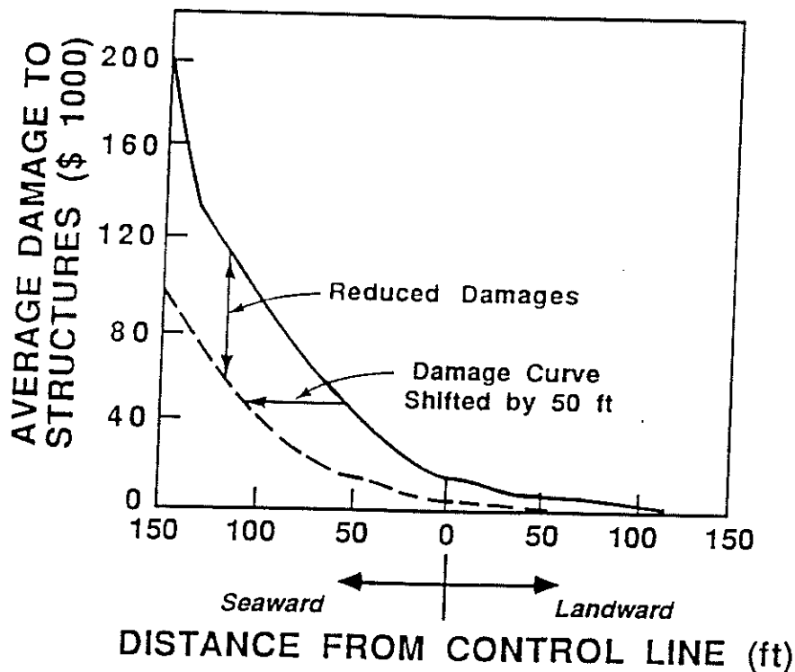
b) Damage Reduction Due to Beach Nourishment Advancing the Profile Fifty Feet Seaward.
