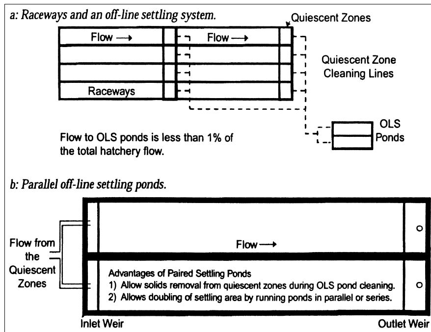
Figure 4.3-4. Offline Settling Ponds
