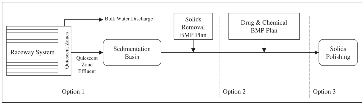
Figure 10.1-1. Flow-through Systems
