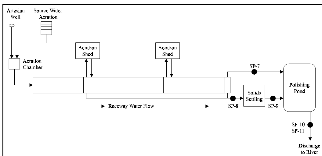
Figure 8.2-2. Schematic of Sampling Points and Facility for Episode 6460
