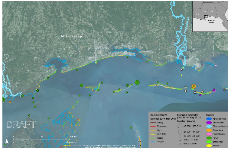
Figure 4.6-62. Maximum SCAT from October 2010, to May 2011, overlaid with sturgeon telemetry data from the same time period. Source rivers are shown in light blue.
