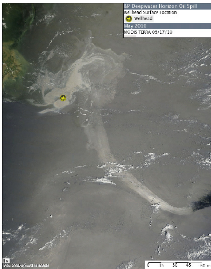
Figure 4.2-14. MODIS image of DWH surface oil on May 17, 2010. On this date, the slick was over 200 miles long (light grey areas).
