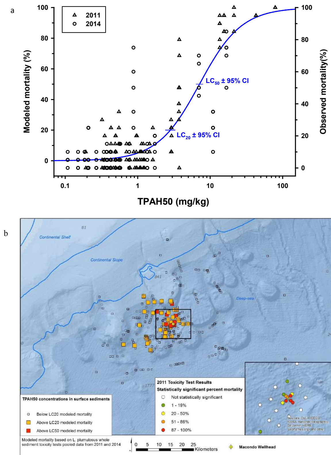
Figure 4.5-10. (a) Sediment toxicity results for deep-sea sediment samples taken in 2011 and 2014 with modeled sediment toxicity indicating LC_{20} and LC_{50} mortality based on TPAH50 values (Krasnec et al. 2015). (b) Map indicating surface TPAH50 concentrations that exceed LC_{20} and LC_{50} values for modeled mortality.
