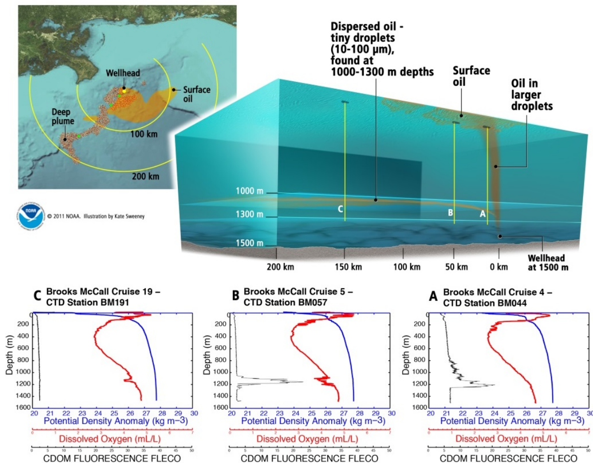
Figure 4.4-19. Oil transport through the Gulf of Mexico water column, illustrating the deep-sea plume and rising oil. The lower figures A-C show conductivity-temperature-depth (CTD) vertical water profiles measured on the Brooks McCall cruises. The depth below the ocean surface is shown on the left side of the profiles; the profiles extend from the bottom of the ocean (at 1,500 meters depth) to the surface. The CTD profiles provide information about the density of the water (blue), the dissolved oxygen content (red), and fluorescence that can indicate the presence of oil (gray). A decrease in dissolved oxygen and an increase in fluorescence at depth indicates the presence of the deep plume.
